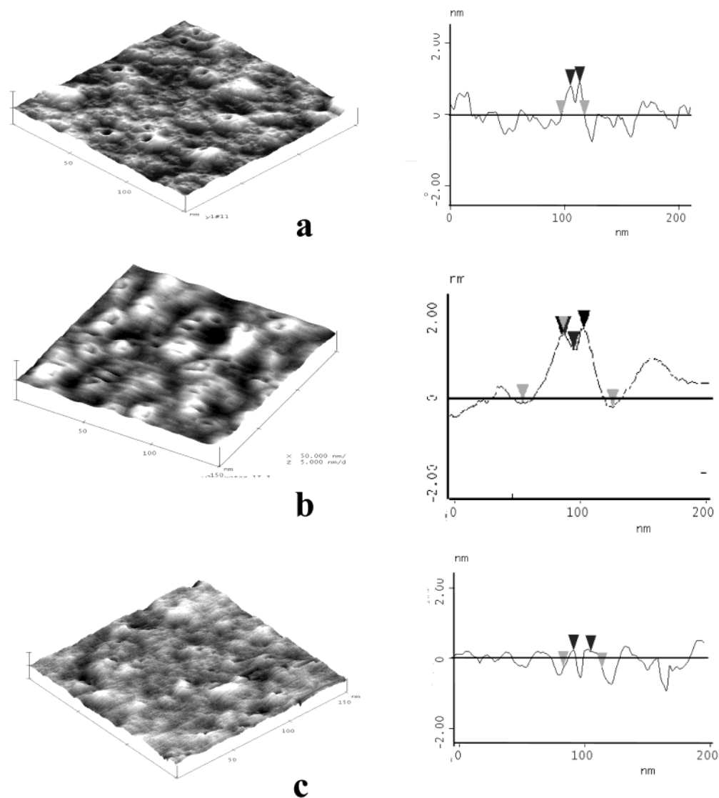
Figure 7. High-resolution 3D AFM images (150 × 150 nm) of craterlike surface micellar structures of the grafted layers of the Y-shaped molecules 1 (a), 2 (b), and 3 (c) and the corresponding cross sections. Z scale is 10 nm for brush 1 and 2 and 6 nm for brush 3 .
